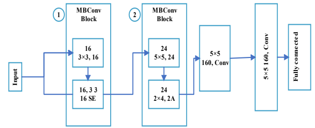
Figure 5. MobileNetV3 Large network architecture A lightweight network optimized for devices with limited processing power.
