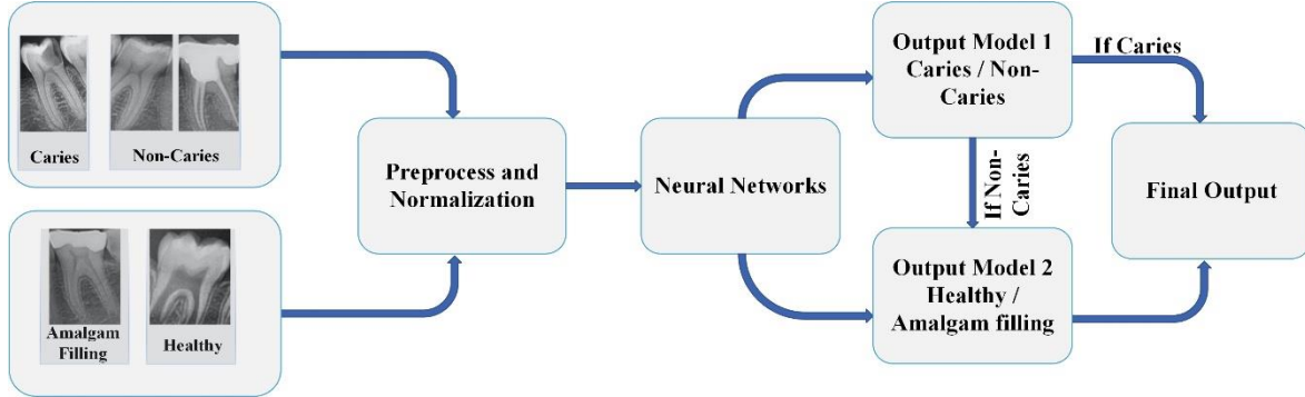
Figure 7. Schematic diagram of the proposed method for hierarchical method of dental images.
